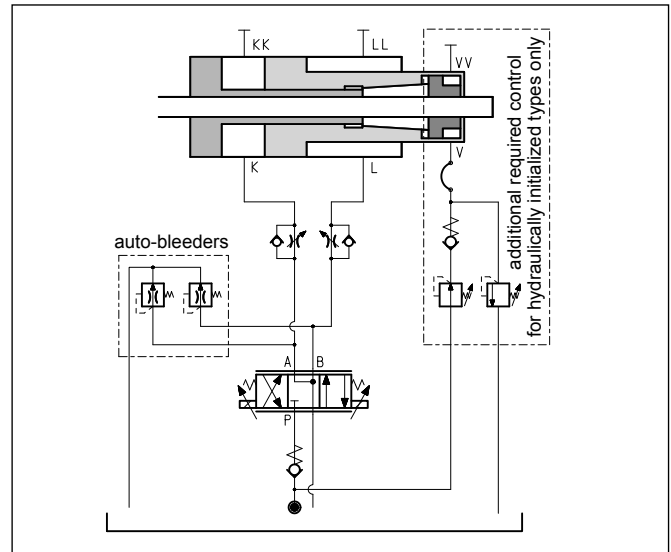
Fig. 4: Principal scheme of control
