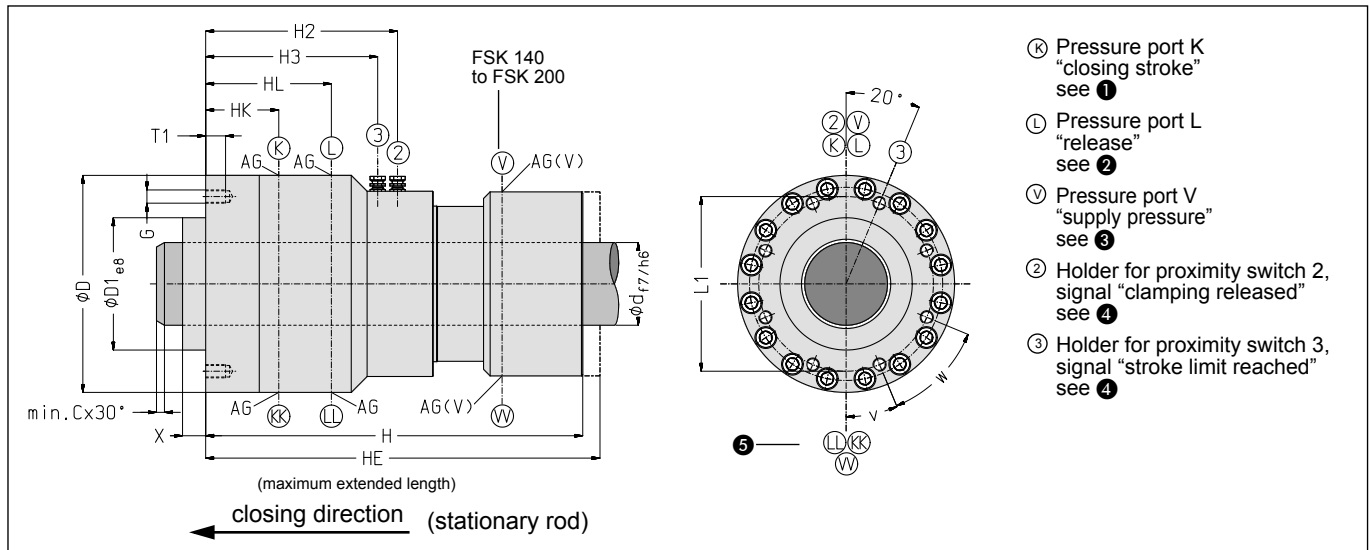
Abb. 5: Dimensions SITEMA PowerStroke series FSK
