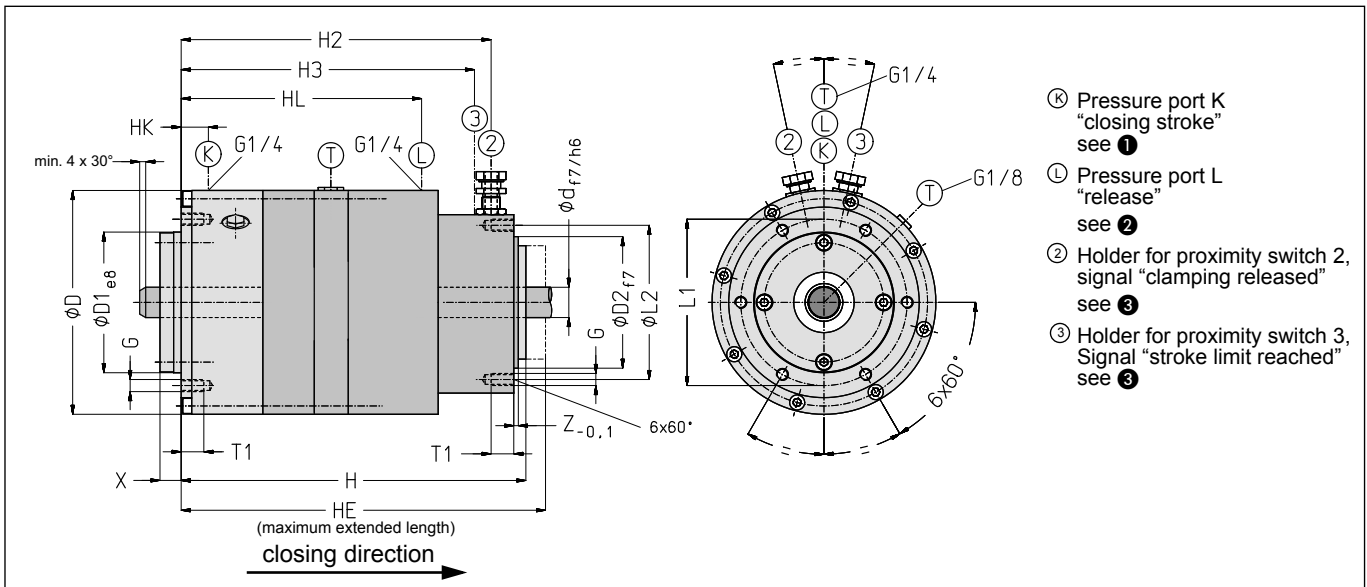
Fig. 5: Dimensions SITEA PowerStroke series FSKP, S types for use with separate rod
